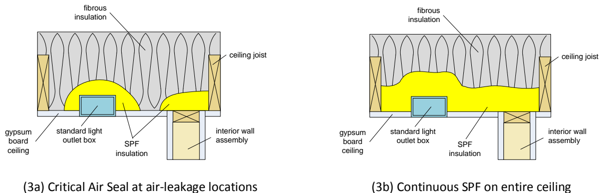
FIGURE 3: HYBRID INSULATION CEILING DESIGNS—ELEVATION SECTION VIEW
