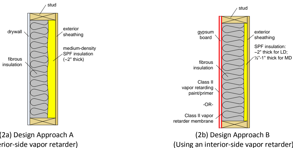
FIGURE 2: HYBRID INSULATION WALL DESIGNS—VERTICAL SECTION VIEW
